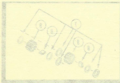
L-60 GEAR ASSEMBLY
