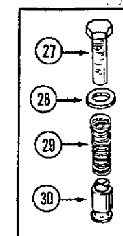
OIL BYPASS VALVE
