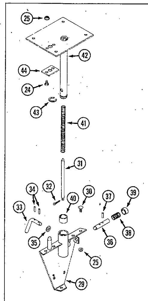
SEAT SUPPORT - 6018BH AND 6018B
