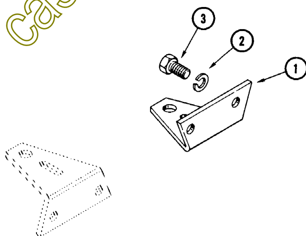
MOUNTING POSITION FOR 220 AND 222 TRACTORS
