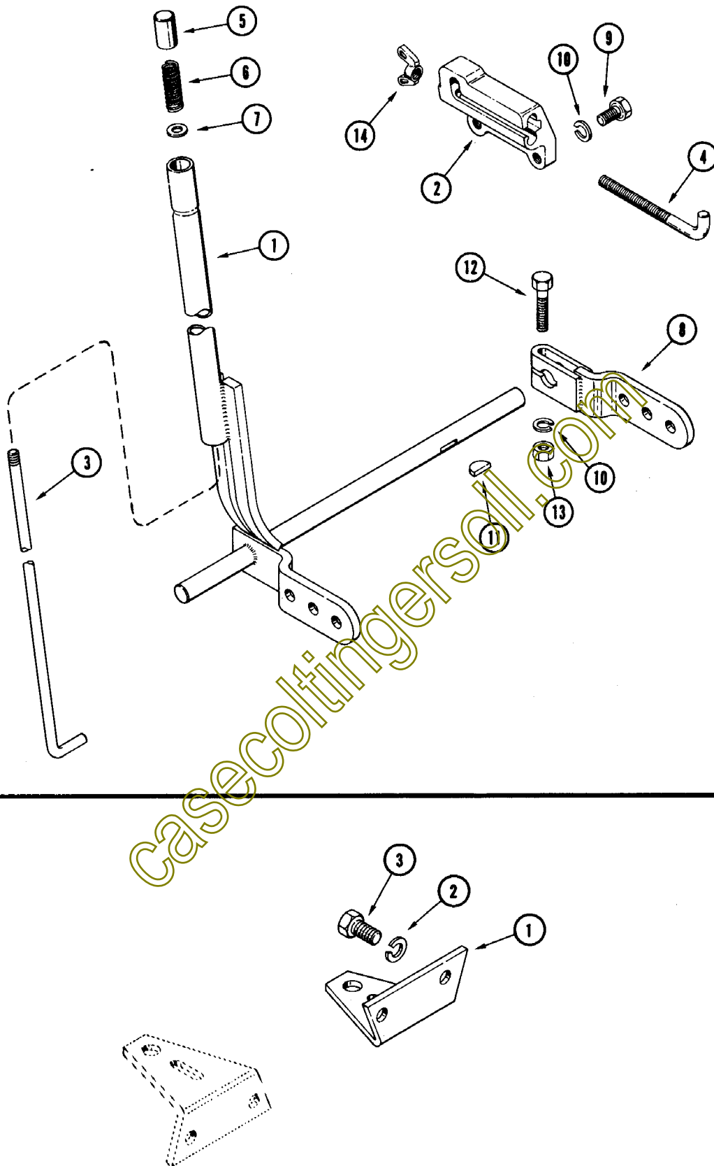
MOUNTING POSITION FOR 220 AND 222 TRACTORS
