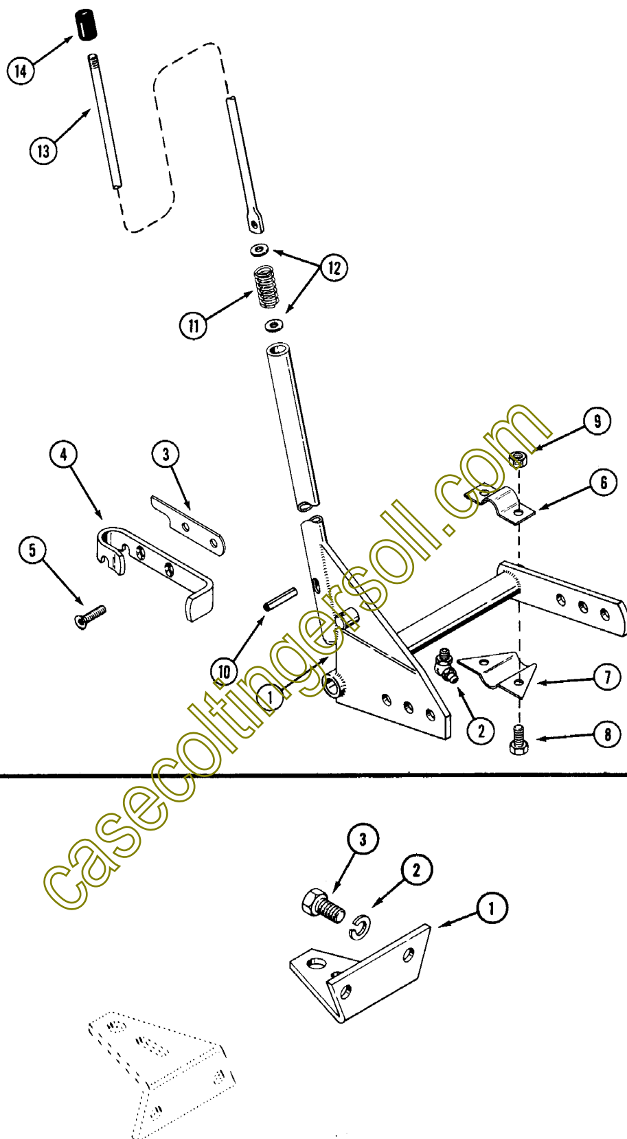
MOUNTING POSITION FOR 220, 222 AND 224 TRACTORS.
