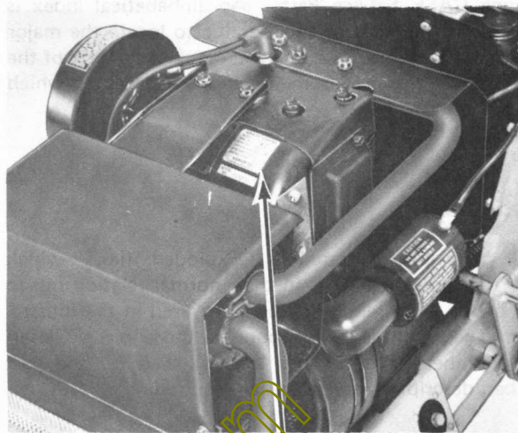
ENGINE MODEL, SERIAL AND SPECIFICATION NUMBER
