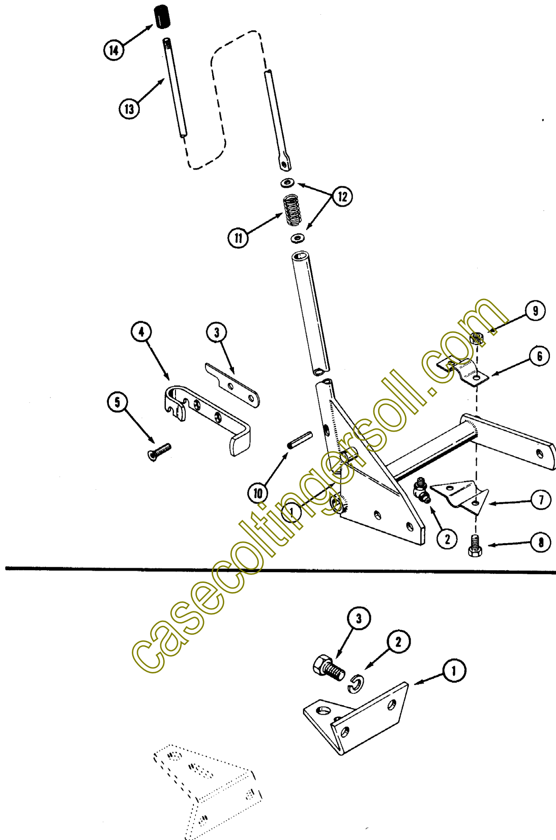
MOUNTING POSITION FOR 220, 222 AND 224 TRACTORS.
